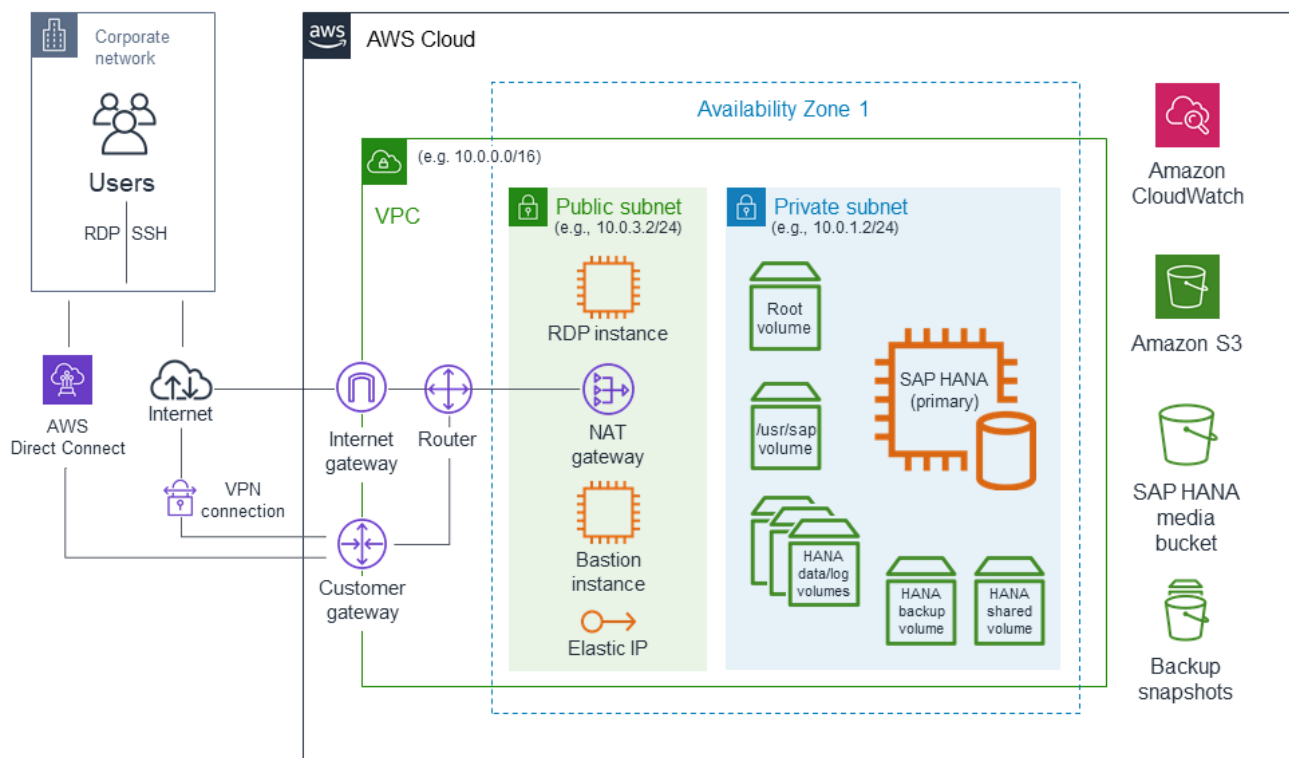
Figure 1: Single-AZ, single-node architecture for SAP HANA on AWS
