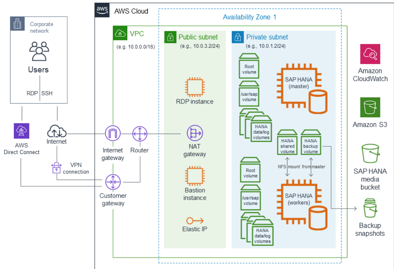
Figure 2: Single-AZ, multi-node architecture for SAP HANA on AWS
